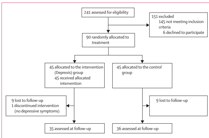
Figure 1: Trial profile
