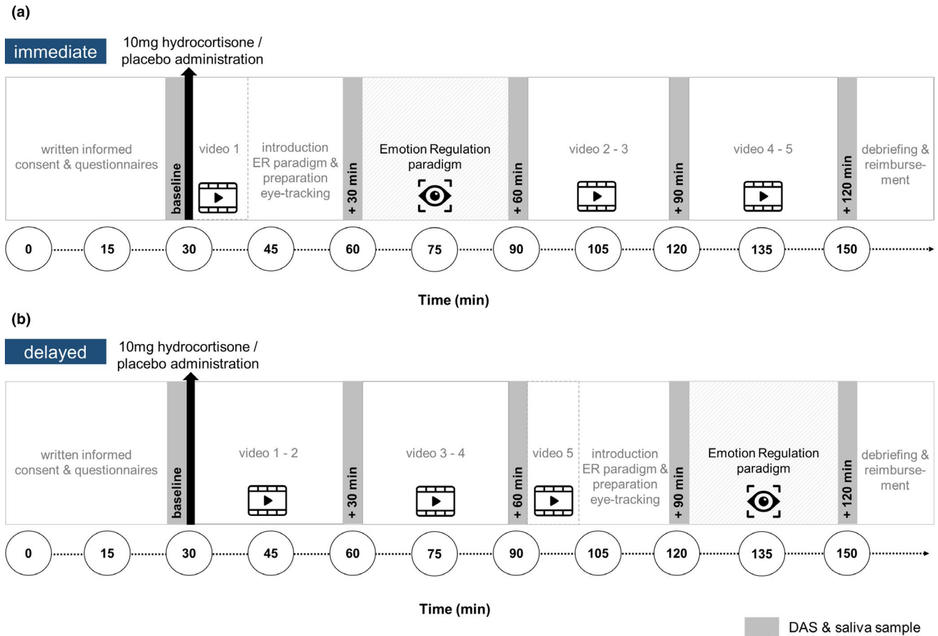
FIGURE 1 Experimental timeline of the immediate (a) and the delayed (b) group. All participants provided five saliva samples together with affective state ratings via the Differential Affective Scale (DAS) over the course of the testing procedure. Sampling time points are marked by shaded areas: baseline, +30, +60, +90 and +120 min after hydrocortisone or placebo administration (time point of pharmacological treatment highlighted by black arrows). The emotion regulation (ER) paradigm started 30 min after the pharmacological treatment for the immediate and 90 min afterwards for the delayed group. Neutral videos were used to bridge the time window between tablet intake and start of the ER paradigm
